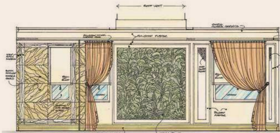
MASTER BATHROOM - ELEVATION B
