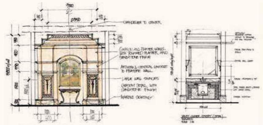
WASHROOMS ENTRANCE - CONCEPT ELEVATION
